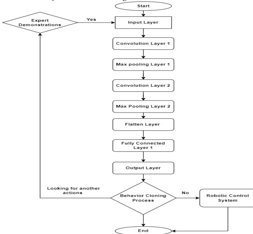
Fig. 2. Flowchart of behaviour cloning for robotic system pick and place
