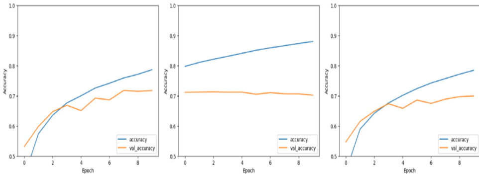
Fig. 4. Testing model customise datasets
