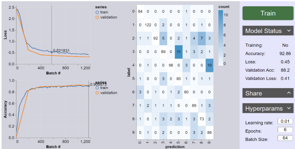
Fig. 3. Training model using CIFAR10 datasets
