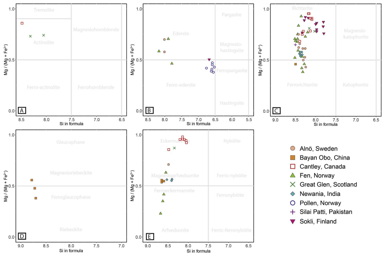
Fig. 9. Classification of amphiboles plotted on graphs of \text{Mg}:\text{Fe}^{3+} ratio and Si calculated in tetrahedral position of formula using the scheme outlined in Leake et al. (1997) and Leake et al. (2004). A: Calcic amphiboles with \text{Ca}_B \geq 1.50 , (\text{Na} + \text{K})_A < 0.50 . B: Classification of calcic amphiboles with \text{Ca}_B \geq 1.50 , (\text{Na} + \text{K})_A \geq 0.50 . C: Classification of sodic-calcic amphiboles with (\text{Na} + \text{K})_A \geq 0.50 . D: Classification of sodic amphiboles with (\text{Na} + \text{K})_A < 0.50 . E: Classification of sodic amphiboles with (\text{Na} + \text{K})_A \geq 0.50 . All data available in Supplementary Table 2. Data sources: Alnö, Sweden (Morogan and Woolley, 1988); Bayan Obo, China (Le Bas, 2008); Cantley, Canada (Hogarth and Lapointe, 1984); Fen, Norway (Kresten and Morogan, 1986; Andersen, 1989); Great Glen, Scotland (Garson et al., 1984); Newania, India (Viladkar and Wimmenauer, 1986); Pollen, Norway (Robins and Tysseland, 1983); Silai Patti, Pakistan (Le Bas, 2008); and Sokli, Finland (Vartiainen and Woolley, 1976).
