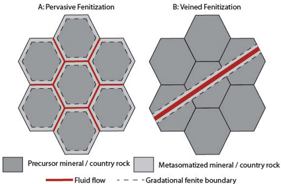
Fig. 6. Schematic diagram illustrating the difference between pervasive fenitization (A) and veined fenitization (B). Fluid interacts with a larger volume of country rock during diffuse porous flow than fluid flowing through fracture.
