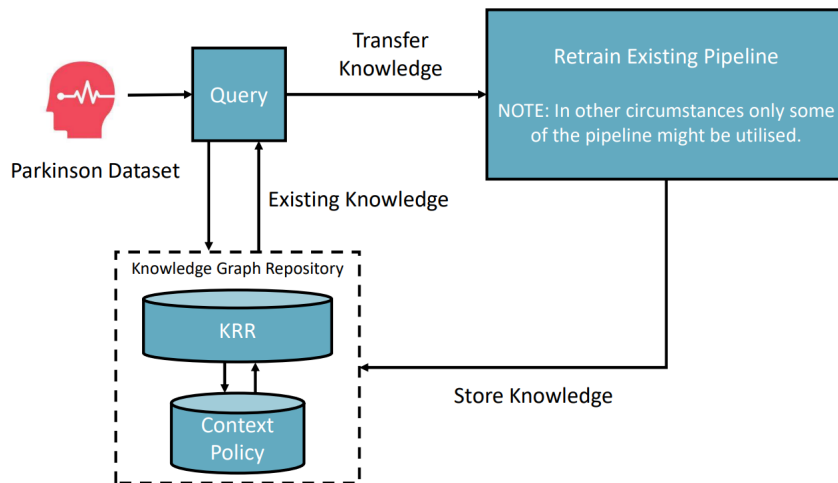
Figure 7. Scenario 2 - Parkinson disease pipeline transfer classification process
