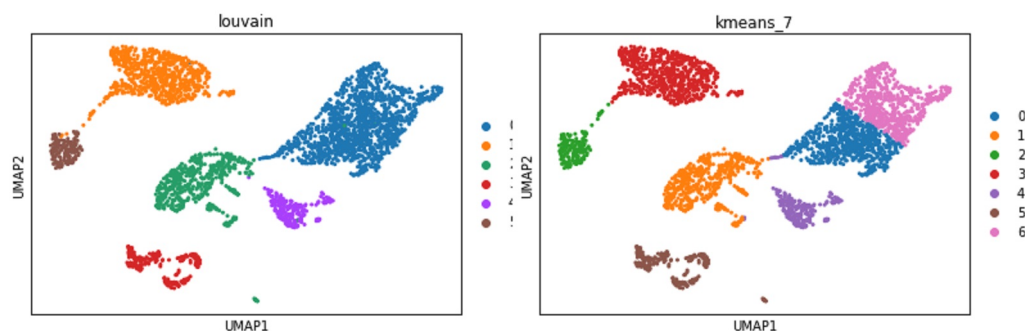
Figure 11. Two clustering outcomes from automatic process
