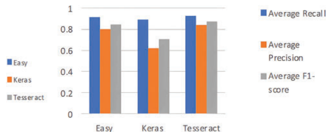
Figure 1: OCR comparison results with Tesseract and Keras-OCR [33]
