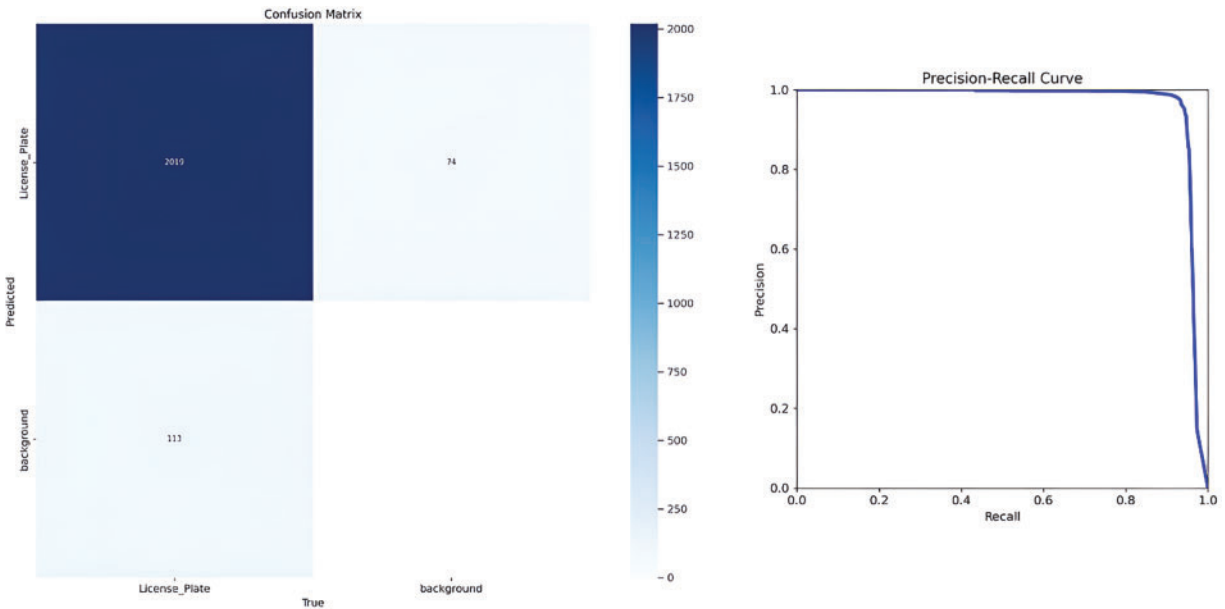
Figure 10: Performance metrics, precision-recall curve, and confusion matrix 8
