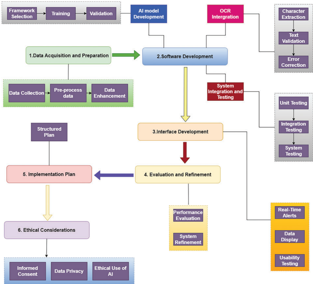
Figure 4: Methodology diagram for AI-driven number plate detection and verification
