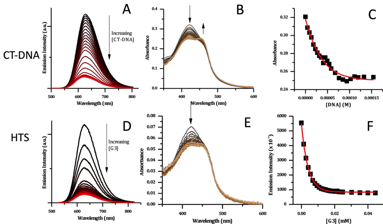
Fig. 7 CT-DNA and HTS titration data for [2]Cl 4 (5 μM concentration, in phosphate buffer A) Changes in emission spectra upon addition of CT-DNA. B) Changes in absorption spectra with CT-DNA. C) Binding curve for the data obtained with CT-DNA based on absorption data– red line shows fit to model developed by Srishailam, et al. 7 D) Changes in emission spectra upon addition of HTS. E) Changes in absorption spectra of [2]Cl 4 upon addition of HTS. F) Binding curve for [2]Cl 4 with HTS based on emission data– red curve shows fitting to a one-set-of-sites binding + non-specific interaction mode.
