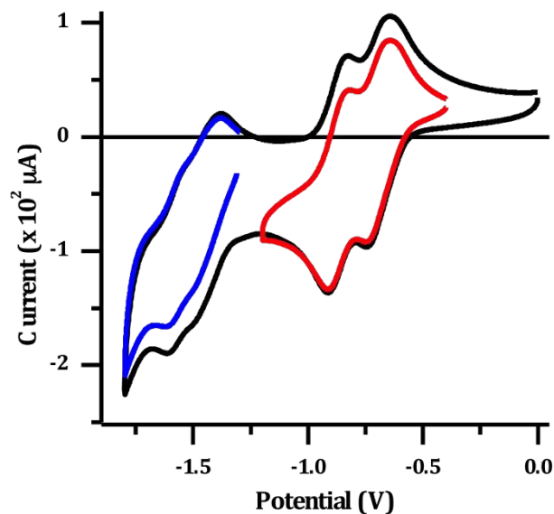
Fig. 3 Cyclic voltammogram for 1 mM [2](\text{PF}_6)_4 in dry DMF with 0.1M \text{N}(\text{n-Bu})_4\text{PF}_6 supporting electrolyte. Red and blue lines show isolated sets of reductions.
