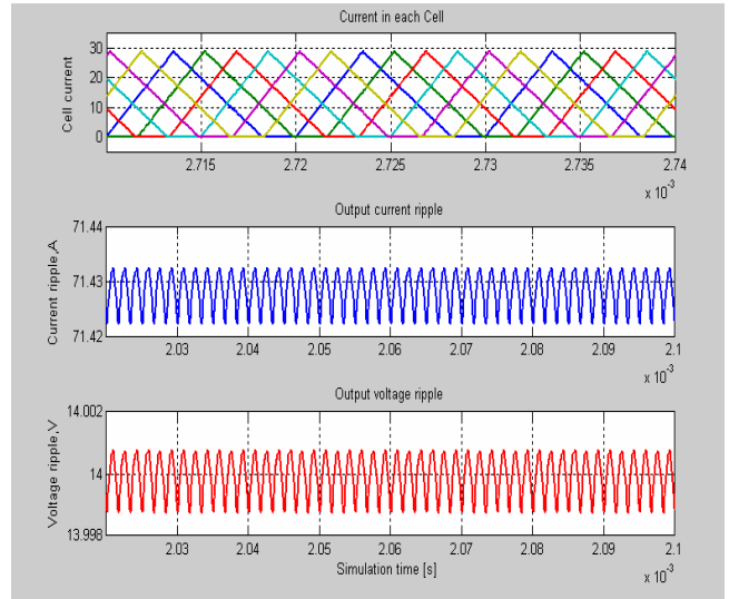
Fig. 10 Current and voltage output ripples
