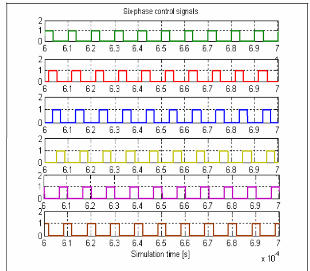
Fig. 8 Six-phase control signals in Simulink
