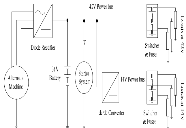
Fig. 1 The 42V/14V system architecture
