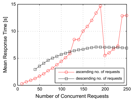
Fig. 6. Measured CxB mean response time with ascending and descending number of context requests.
