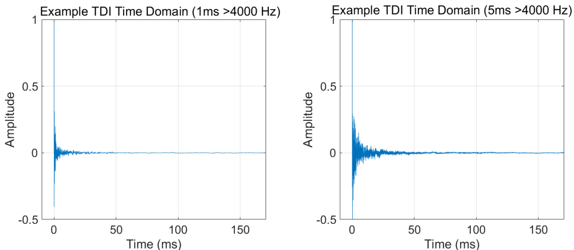
Figure 2.1 Example TDIs. Each TDI was generated with the same decay constants (Table 3.1) except the left plot shows TDI generated with all cosine waves above 4000 Hz set to 1 ms decay, and the right plot shows the result of setting these cosine waves to 5 ms decay. The increased amplitude of the noise tail in the right plot equates to greater decorrelation when multiple TDIs are used, but also greater audibility of the filter.
