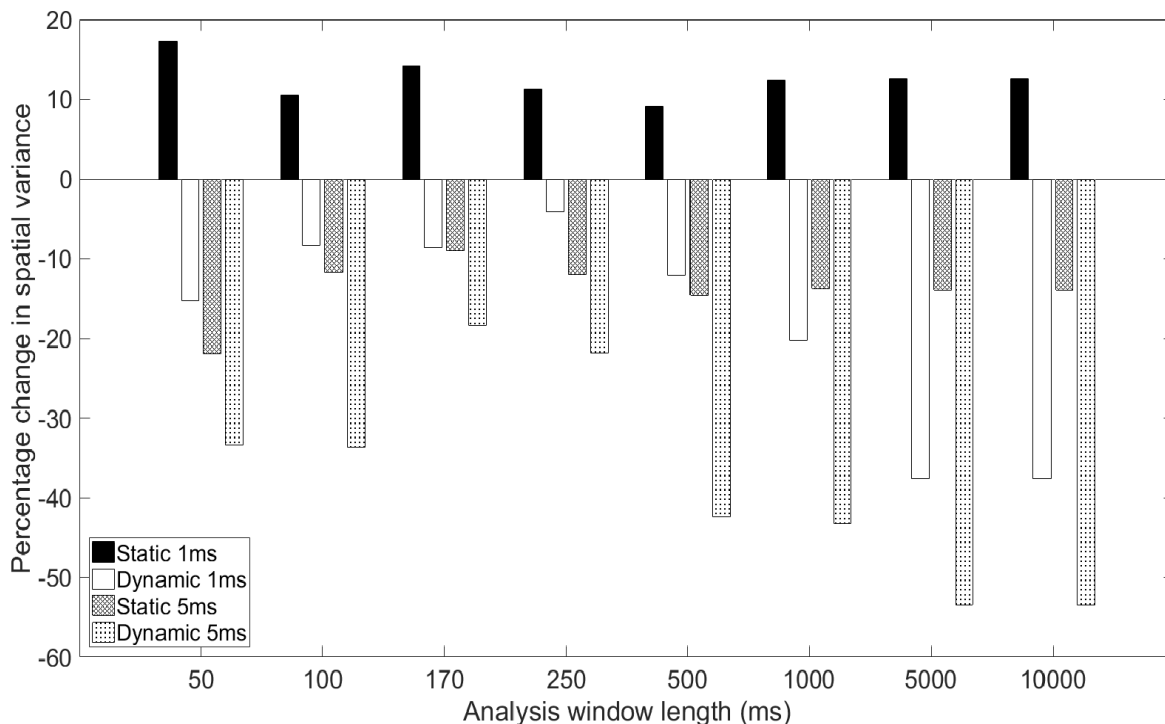
Figure 2.2 Percentage change in SV for static and dynamic DiSP using both 1 ms and 5 ms TDI libraries for analysis windows ranging from 50 ms to 10 s
