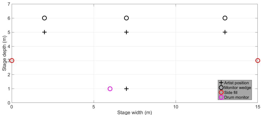
Figure 3.1 Example monitor speaker/performer location set up used for simulation In this test, an example stage set up was simulated. Six loudspeakers were positioned as in Figure 3.1. To simulate an outdoor setting, only the floor (stage) of the model was made reflective, and all other surfaces were set to anechoic. The frequency response measurements were generated in the same way as the other tests, over the course of 1 s. Dynamic DiSP was used up to 4 kHz, again by setting decay times above this at 1 ms, and results are shown from 0-4000 Hz.
