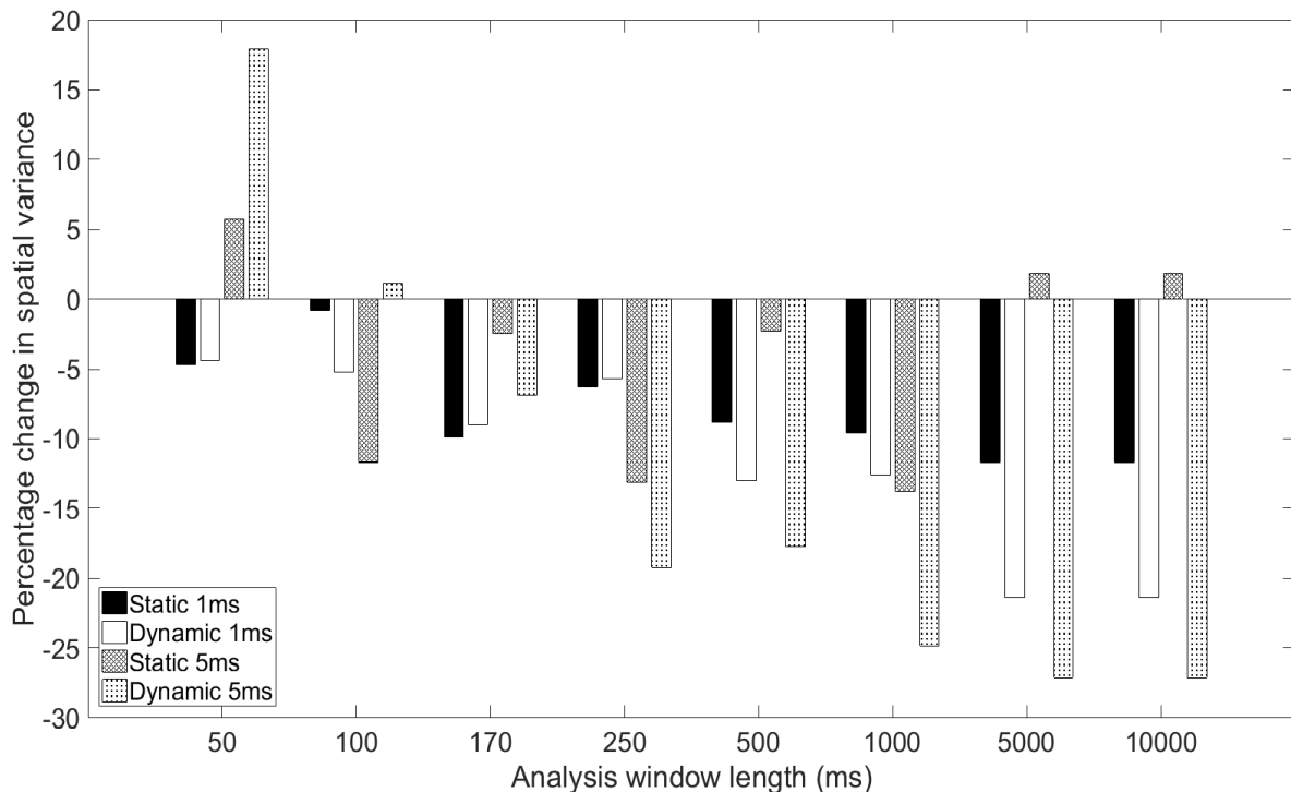
Figure 2.4 Percentage change in SV for static and dynamic DiSP using both 1ms and 5ms TDI libraries for analysis windows ranging from 50ms to 10s with a single source.
