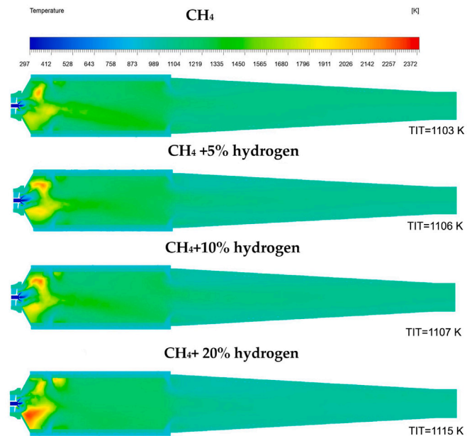
Fig. 3. Temperature profile contours at the same midplane of the combustor fed with \text{CH}_4 , \text{CH}_4 + 5\% \text{H}_2 , \text{CH}_4 + 10\% \text{H}_2 , and \text{CH}_4 + 20\% \text{H}_2 .
