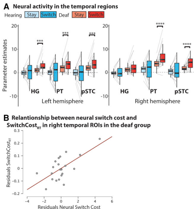
Figure 4 Switching task analysis. (A) Neural activity in temporal ROIs. *** P < 0.005 ; **** P < 0.001 . (B) Partial correlation plot between SwitchCost_{RT} and neural switch cost in right temporal ROIs in the group of deaf individuals. Partial correlation from a multiple linear model with SwitchCost_{RT} as the dependent variable and the following covariates: right hemisphere neural switch cost, left hemisphere neural switch cost, and language.
