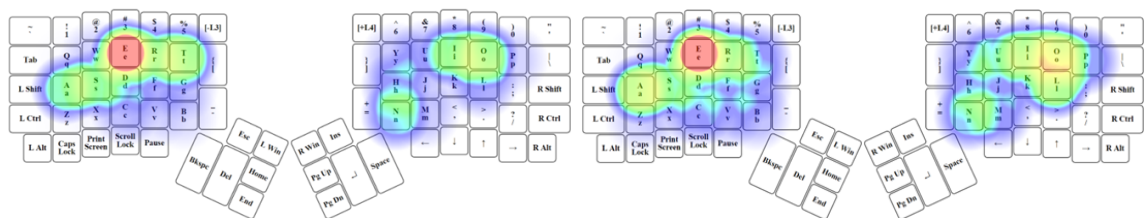
(a) A heatmap of the phrase set from [28]. (b) A heatmap of the generated phrase set.
