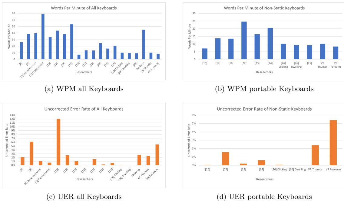
Fig. 3: Comparison to other keyboards.
