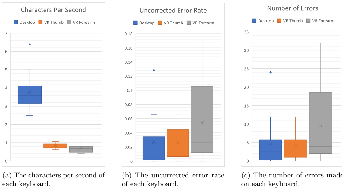
Fig. 2: Box and whisker plots showing the results of the keyboards.
