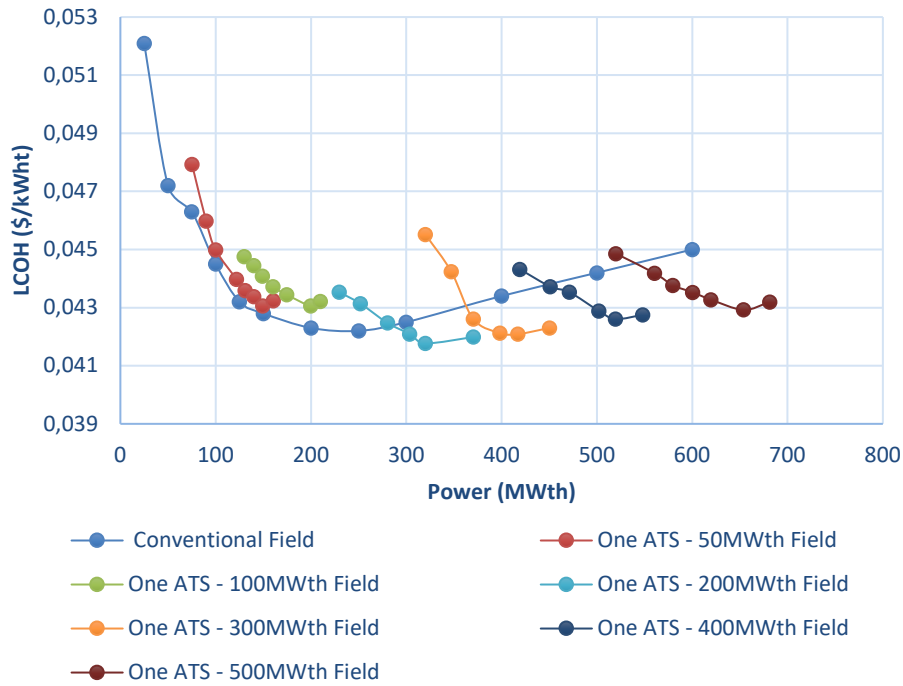
Figure 5. LCOH for conventional field and one ATS configuration at different thermal
